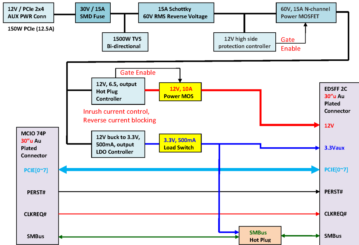
GE0185A MCIO 74P/PCIe 5.0 to EDSFF 2C adapter Block Diagram
