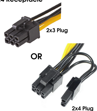
2x4 Plug Mating with a 2x4 Receptacle
