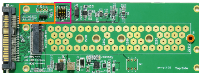
Model No.: GD1401A U.2 (SFF-8639) PCIe Gen 4 to M.2 NVMe SSD Adapter
