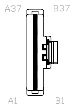
CN2 SLIMLINE 74 PIN X8 PLUG (SFF-8654)
